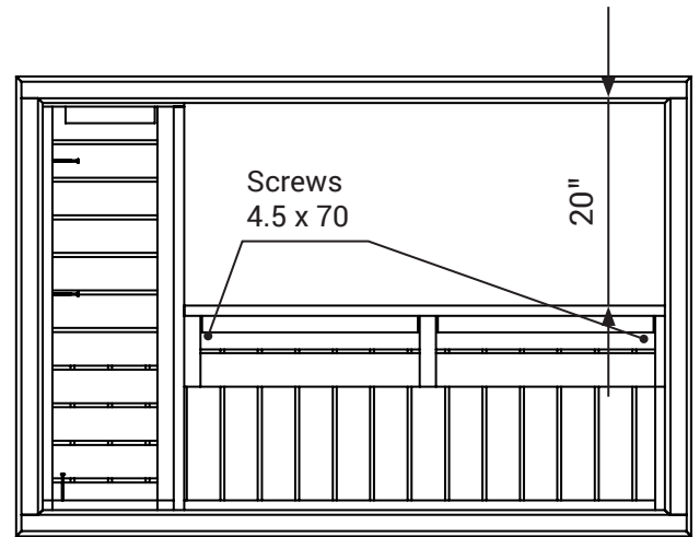
Floorplan View
