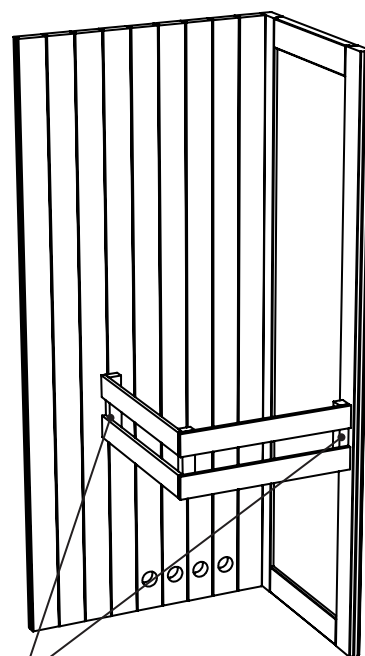
Screws 4 x 60
